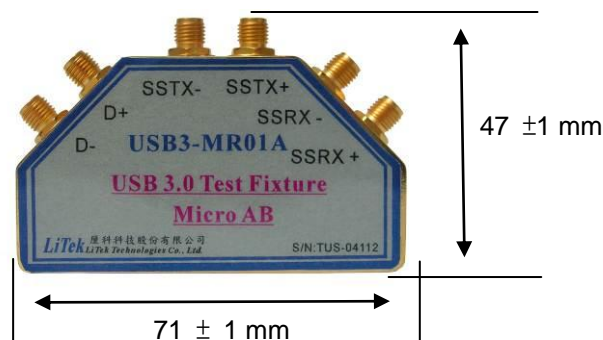
Fig4: USB3-MR01A dimensions
