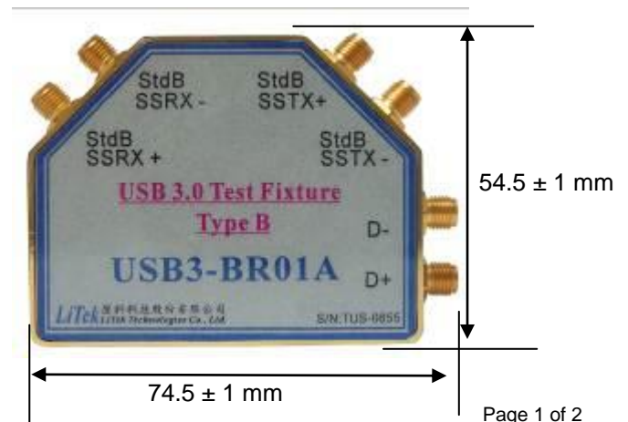
Fig4: USB3-BR01A dimensions
