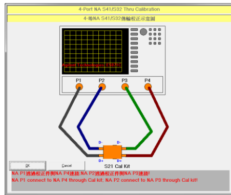
Fig3: USB3-CK03AR-USB3.0 software Calibration.
