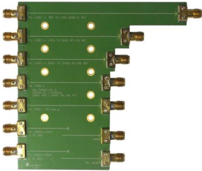
Fig1: USB3.0 2X Trace TRL Calibration Fixture(USB3-CK03AR)
