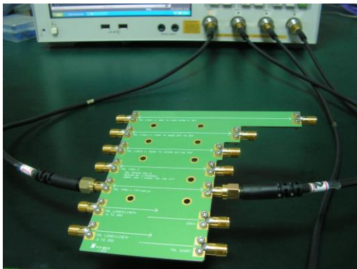
Fig2: USB3-CK03AR connect with SMA Coaxial cable form Equipment for calibration before testing.
