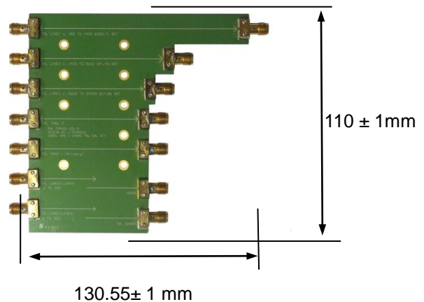
Fig4: USB3-CK03AR dimensions
