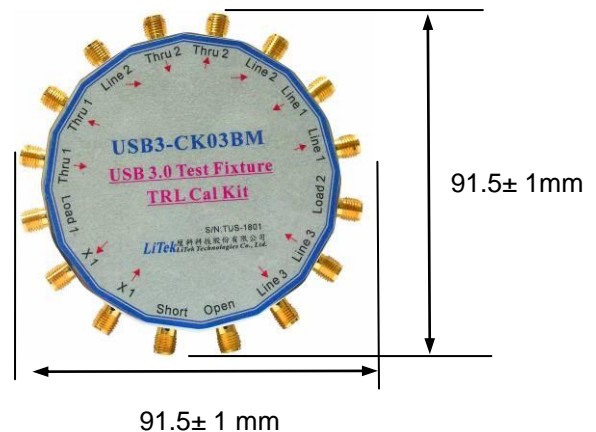
Fig4: USB3-CK03BM dimensions
