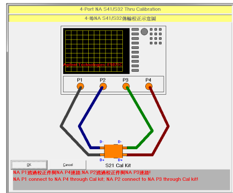
Fig3: USB3-CK03BM-USB3.0 software Calibration.
