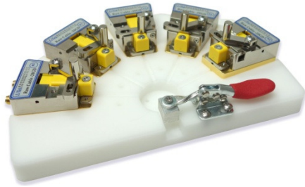
Figure 1: LT-100R-20GD-5P 5pair Raw Cable Test Fixture
