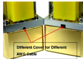
Figure 4: Different cover for Different AWG Cable
