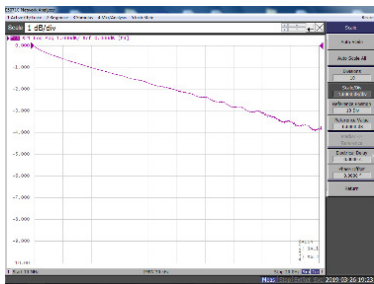
Figure 2: The SDD21 of Calibration Kit
