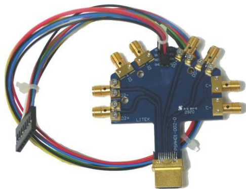
Figure1: HDMI-AP03AR(HAD-13) HDMI Probe test fixture and extended cable.
