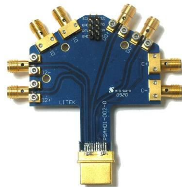
Figure2: HDMI-AP03AR(HAD-13) HDMI Probe Test Fixture
