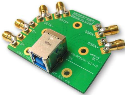
Fig1: USB3.0 CTS Type B receptacle Test Fixture(USB3-BR03AR)
