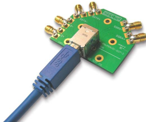
Fig3: USB3-BR03AR plugged with Type B Plug DUT.
