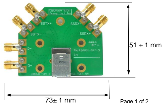
Fig4: USB3-BR03AR dimensions
