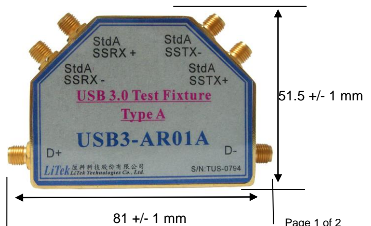
Fig4: USB3-AR01A dimensions
