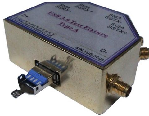
Fig3: USB3-AR01A plugged with Type A Plug DUT.
