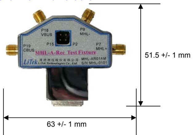
Fig4: USB3-AR01AM dimensions
